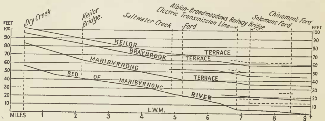
FIG. 5. Profile of Surfaces of Terraces and Bed of Maribyrnong River between Dry Creek and Chinaman's Ford.
